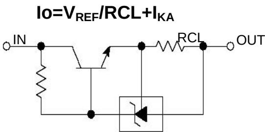
Constant Current Source TL431M
